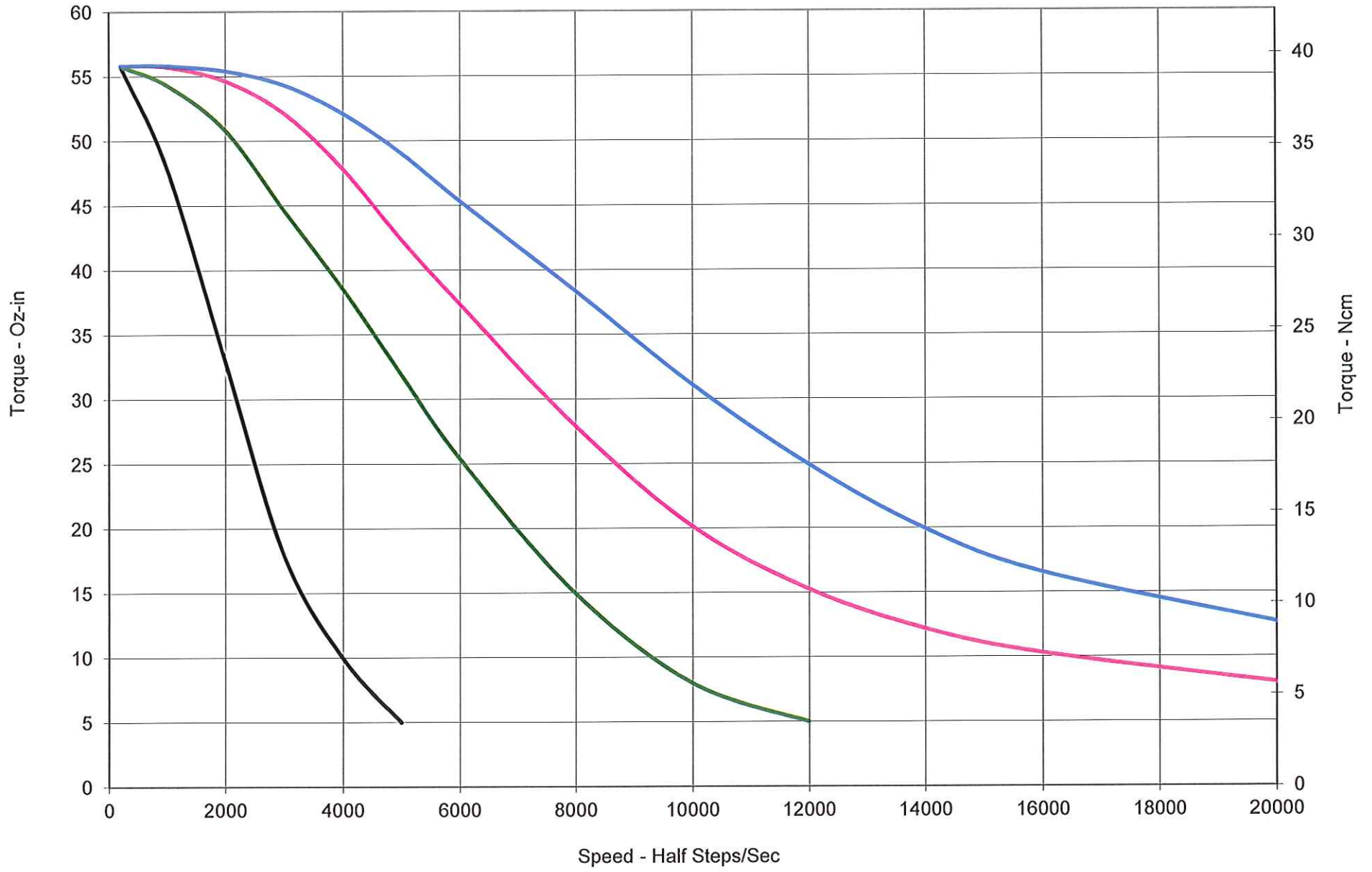
TPE17M-44A15 - Constant Current Drive - 1.5 Amps RMS
