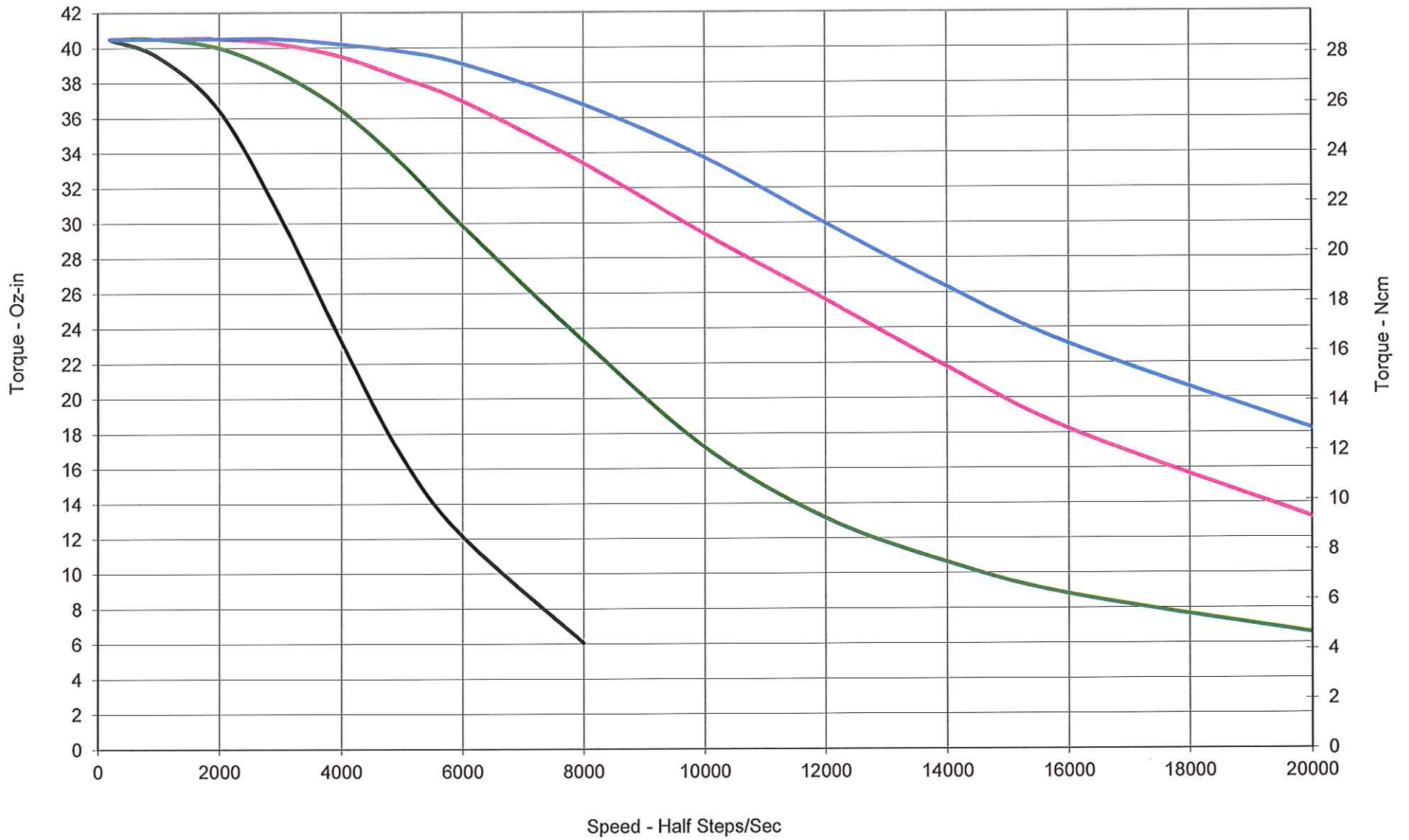
TPE17M-32A20 - Constant Current Drive - 2 Amps RMS
