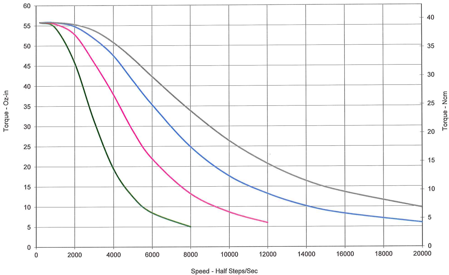
TPE17M-44A10 - Constant Current Drive - 1 Amp RMS
