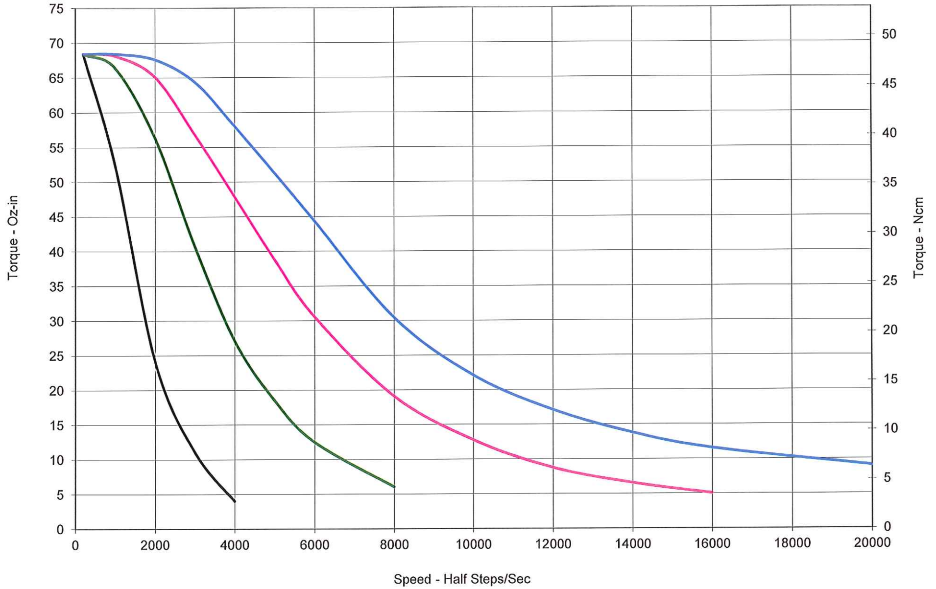
TPE17M-55A15 - Constant Current Drive - 1.5 Amps RMS
