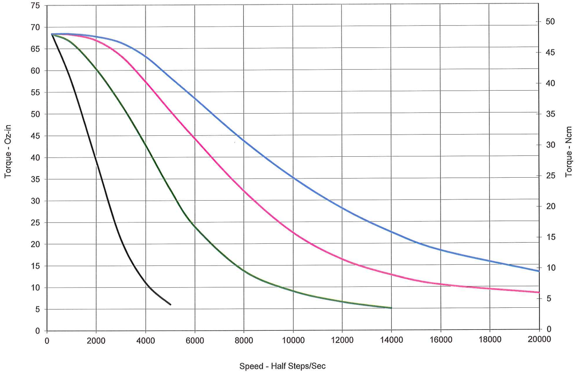
TPE17M-55A20 - Constant Current Drive - 2 Amps RMS
