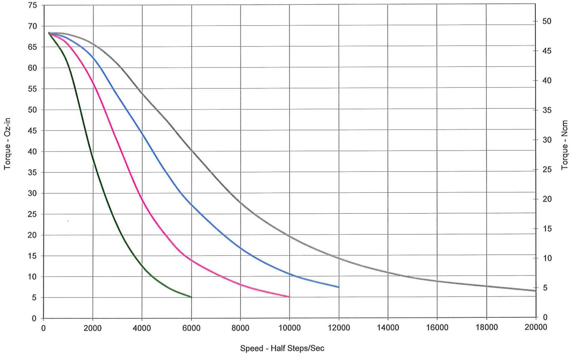
TPE17M-55A10 - Constant Current Drive - 1 Amp RMS
