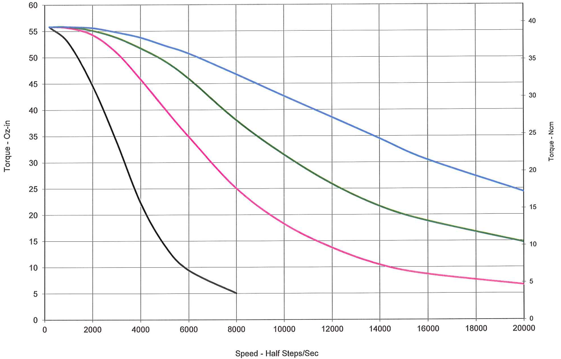
TPE17M-44A20 - Constant Current Drive - 2 Amps RMS
